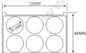
ES1060H-6Y36 ES1060HW-6Y36 ES1060P-6Y36
