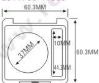
ES1173-1Y36S ES1173P-1Y36S ES1173C-1Y36S
