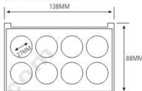
ES1060H-8Y27NS ES1060HW-8Y27NS ES1060P-8Y27NS
