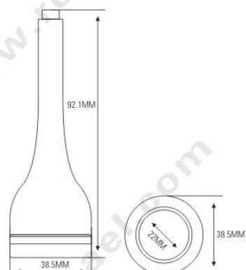
LP0036-1 SIZE: Ø38.5×H92.1mm
