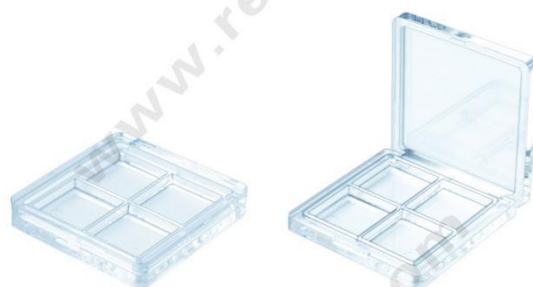
ES1186-4F SIZE: L61xW60.9xH10.9mm
