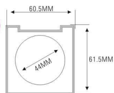
★ MAGNETIC OPENNING & CLOSE (磁性开关) ES1160M-1Y44(ES1160BY-44NT) SIZE:L60.5xW61.5xH14.7mm
