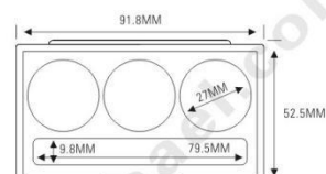
★ MADE OF PP MATERIAL (材质为PP料) ES6003-3Y27S SIZE: L92xW52.5xH11.8mm
