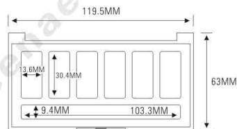
ES1179W-6F ES1179H-6F ES1179HW-6F
