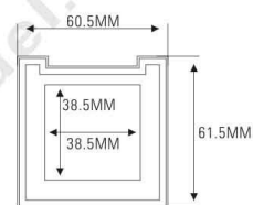
★ MAGNETIC OPENNING & CLOSE (磁性开关) ES1160M-1F(ES1160BF-NT) SIZE:L60.5xW61.5xH14.7mm
