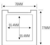
ES1181F-1F (有中格 W/ TRAY) ES1181WF-1F (有中格 W/ TRAY)
