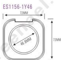
ES1156-1Y46 ES1156-4Y-HAA SIZE: L72xW72xH20.3mm
