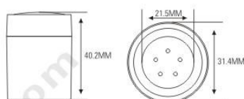
LP0005 SIZE: Ø31.4×H40.2mm
