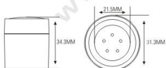
LP0006 SIZE: Ø31.3×H34.3mm
