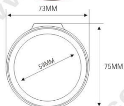
★ MADE OF PP MATERIAL (材质为PP料) ES6001 SIZE: L73xW75xH14.2mm
