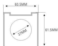
★ MAGNETIC OPENNING & CLOSE (磁性开关) ES1160WM-1Y37(ES1160WY-37NT) SIZE:L60.5xW61.5xH14.7mm
