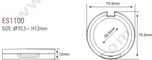
ES1100 SIZE: Ø70.5 × H12mm
