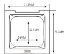
ES1081B SIZE: L71.3xW71.3xH19.7mm
