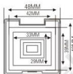
ES1058 SIZE: L48xW48xH13mm
