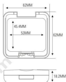
ES1020 SIZE: L62 \times W62 \times H18.2\text{mm}
