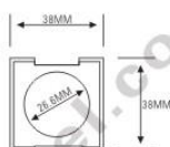
ES1131 SIZE: L38×W38×H13.9mm
