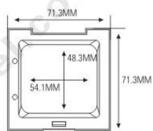
ES1081 SIZE: L71.3xW71.3xH19.7mm
