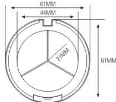
ES1014A-3 SIZE: Ø61×H20.5mm
