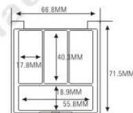
ES1146-3F SIZE: L66.8×W71.5×H12.2mm
