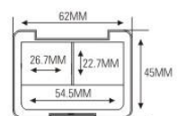
ES1052 SIZE: L62×W45×H13.2mm
