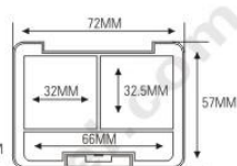
ES1051-2 ES1051-4 SIZE: L72×W57×H15.5mm
