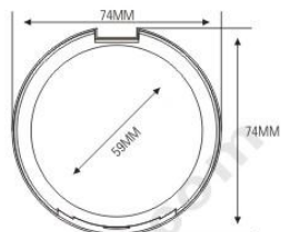
ES1050-4 SIZE: \varnothing 74 \times H17.5\text{mm}
