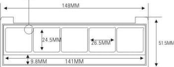
ES1011-5FTSNB(ES1011C-5FY) SIZE: L148×W51.5×H12.5mm
