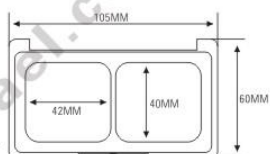
ES1143-2Y SIZE: L105×W60×H11.7mm
