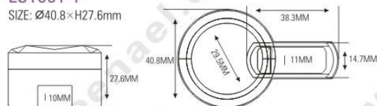
ES1001-2 SIZE: Ø40.8 × H27.6mm
