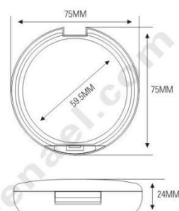
ES1041 SIZE: \varnothing 75 \times H24\text{mm}
