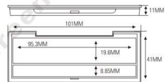
ES1077 SIZE: L101×W41×H11mm
